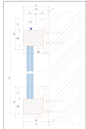
Abb. 8.64: GM WINDOORAIL®
